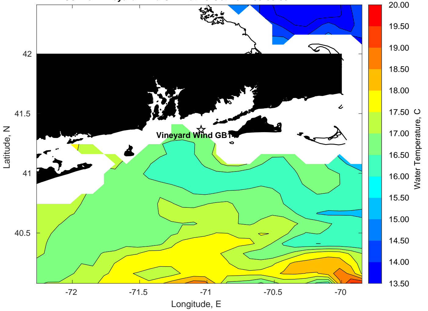
SST for Vineyard Wind GB14 at 13-Oct-2022 00:00:00
